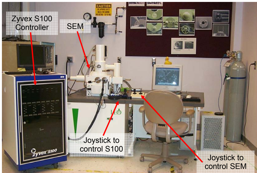
Figure 4.1. The Zyvex Nanomanipulation System
