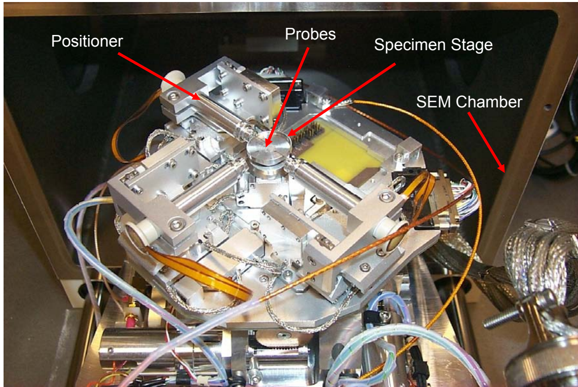
Figure 4.2. Zyvex S100 Mounted on SEM Stage
