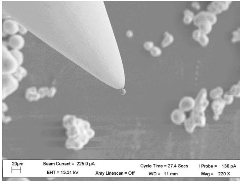
Figure 4.6. Particle Attached to Probe Using DEP
