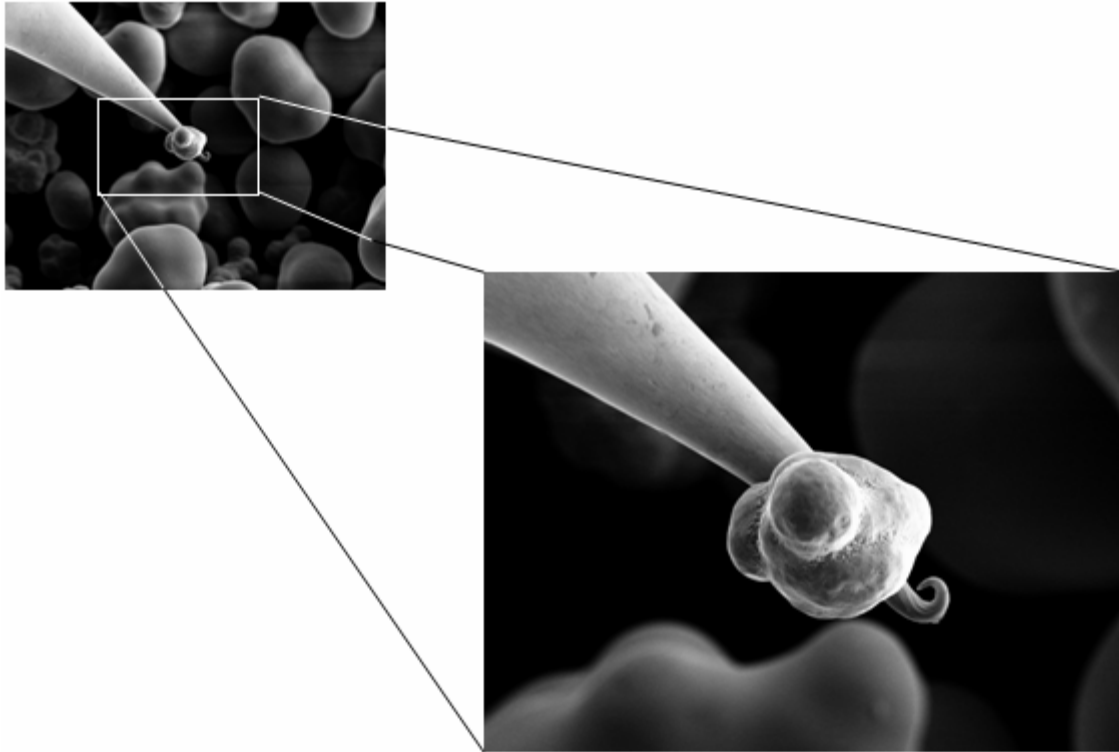
Figure 4.5. Nickel Particle Lifted by Zyvex Probe
