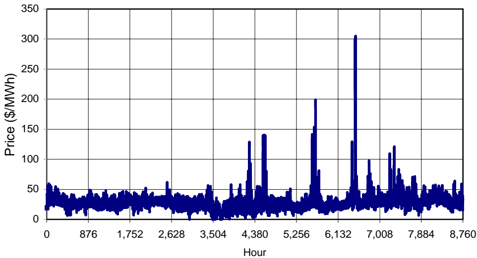
Figure 5. Chronological Electricity Price Data for California, 2004 (projected)
