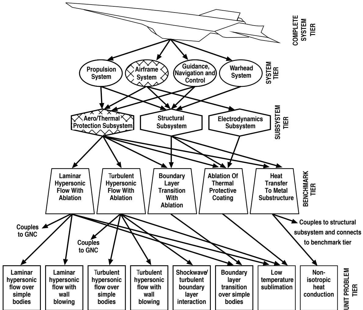
Figure 10 Validation Hierarchy for a Hypersonic Cruise Missile[147]
