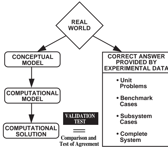
Figure 3 Validation Process[3]
