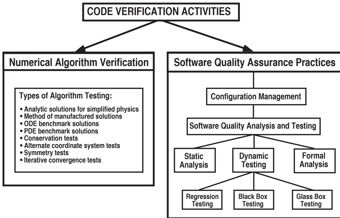
Figure 8 Integrated View of Code Verification in Computational Physics (Adapted from Refs. [148])
