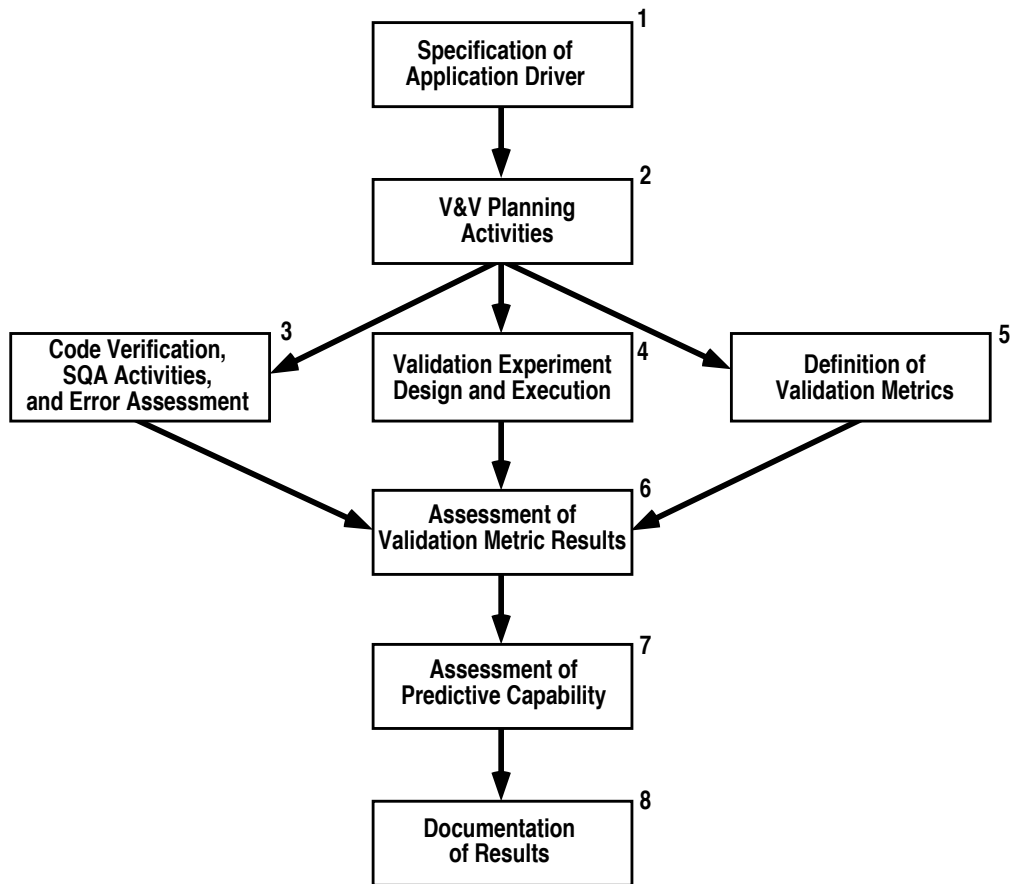
Figure 6 Verification-Validation-Predictive Process (Adapted from Ref. [190])
