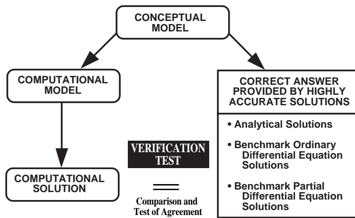
Figure 2 Verification Process[3]
